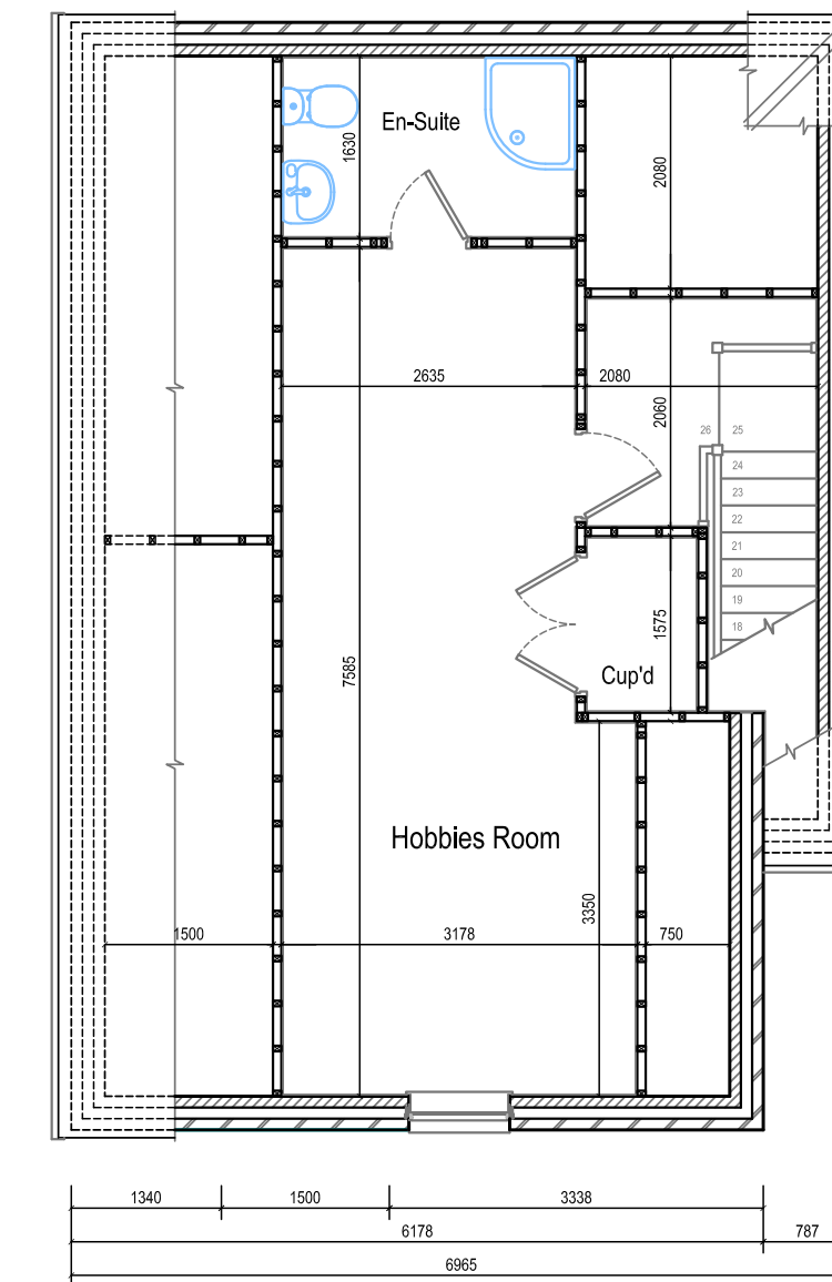
Second Floor / Roofspace Plan
